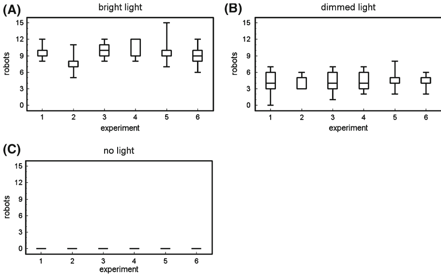
Fig. 11 (a) Number of aggregated robots per interval in a static environment with one bright light (1,100 lux) in the arena. Approx. 60% of all robots aggregated under this environmental condition. (b) Number of aggregated robots per interval in a static environment with one dimmed light (390 lux) in the arena. Approx. 30% of all robots aggregated under this environmental condition. (c) Number of aggregated robots per interval in a static environment without any light source. This environmental condition always resulted in no aggregation of robots. Medians, quartiles, and extremes are depicted. N = 6 repetitions with nine sampling intervals each
