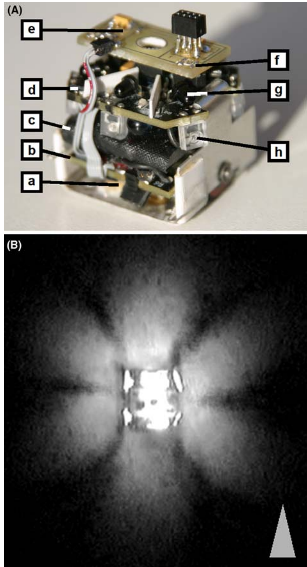
Fig. 9 Top: The Jasmine-III robot, front side: (a) one of the two motors; (b) motion-control-board for compensating manufacturing differences of the motors; (c) lithium-polymer accumulator; (d) main board; (e) illuminance-sensor-board; (f) single light sensor on light-board; (g) IR-sensor for distance measurement; (h) IR-emitter, corresponding with IR-sensor. Bottom: IR-image of a single robot. Arrow indicates heading of robot
