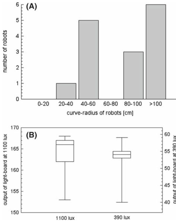
Fig. 10 (a) Distribution of the robots' side-drifts. Most robots (9 of 15) had no, or only a very slight drift aside with curve-radii greater than 80 cm. Some robots (6 of 15) had a curve radius of less than 60 cm and more than 20 cm. No robot had a curve radius below 20 cm. (b) Median, quartiles and extreme values of measured light intensities (reported sensor values) under constant controlled conditions (1,100 and 390 lux)
