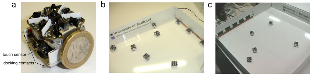
Fig. 1. (a) The “Jasmine” microrobot’s recharging contacts. The touch sensor on the front of the robot is also shown. (b) The first docking station, at which each robot can become a communication point. (c) The second docking station, with integrated communication points.
