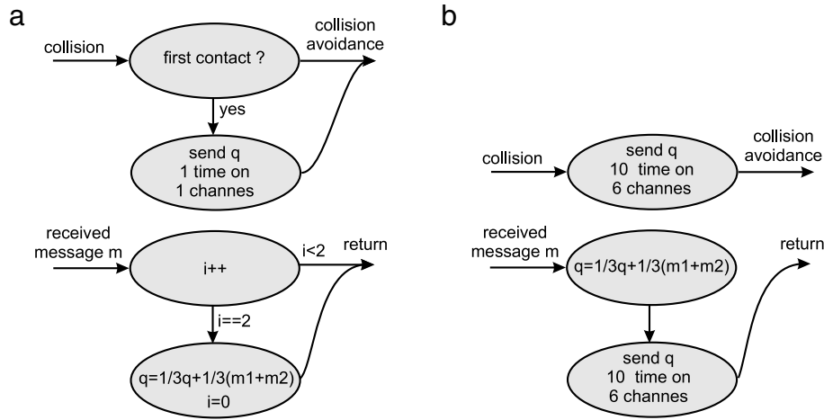
Fig. 5. (a) Slow information update, where the message triggering averaging is sent only once, on collision with another robot. (b) Fast information update, where the messages are sent continuously.
